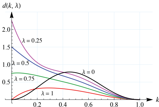
Figure 2: The function k \mapsto d(k, \lambda) , when 0 \leq k \leq 1 for \lambda = 0, 1/4, 1/2, 3/4, 1
