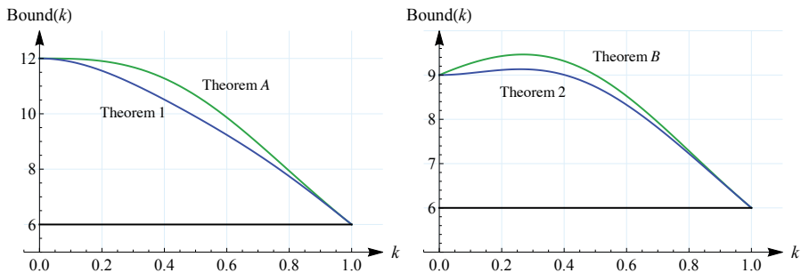
Figure 1: Bounds obtained by Theorem A and Theorem 1 (left) and by Theorem B and Theorem 2 (for \lambda = 1 ) (right) when 0 \leq k \leq 1
