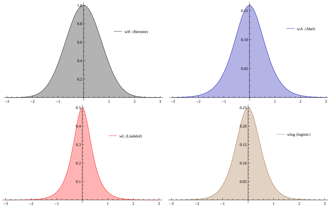
Figure 2: Weight functions on \mathbb{R} : Cases 1°–4°
