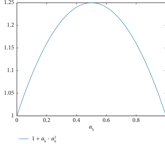
FIGURE 1: The graph of the function \mathfrak{I}(\alpha_k) = 1 + \alpha_k - \alpha_k^2 for \alpha_k \in (0, 1] .
