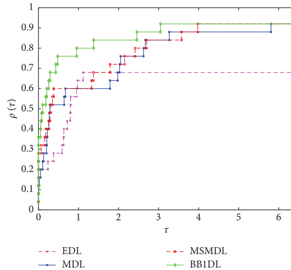
FIGURE 5: CPUts performance profiles for EDL, MDL, MSMDL, and BB1DL.
