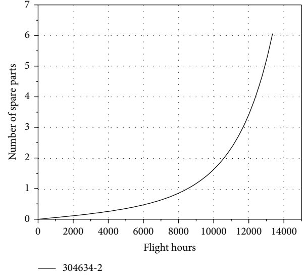
FIGURE 5: Number of spare parts in function of time for part 304634-2.
