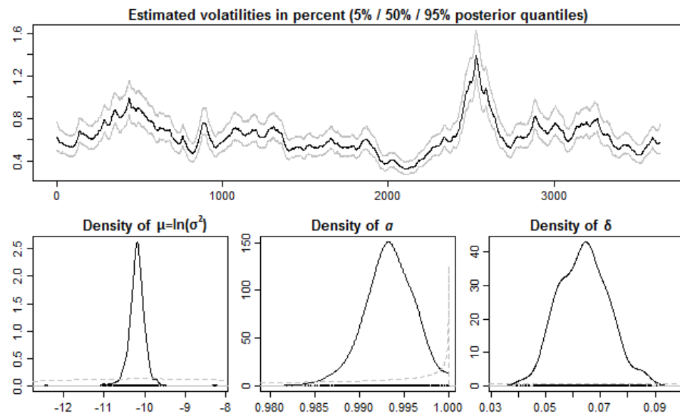
FIG. 5.3: Estimations of SV-parameters obtained by MCMC method (dataset is time series of daily returns of the exchange rates of USD per one euro).
