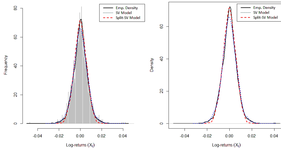
FIG. 5.5: Empirical and fitted log-returns densities of the exchange rates of USD per one euro
