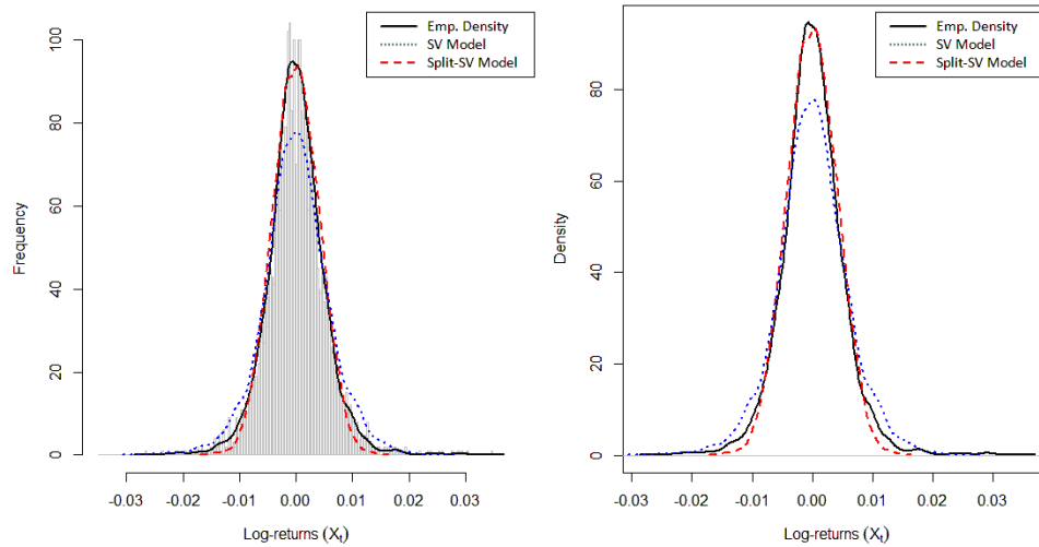
FIG. 5.4: Empirical and fitted log-returns densities of the exchange rates of GBP per one euro
