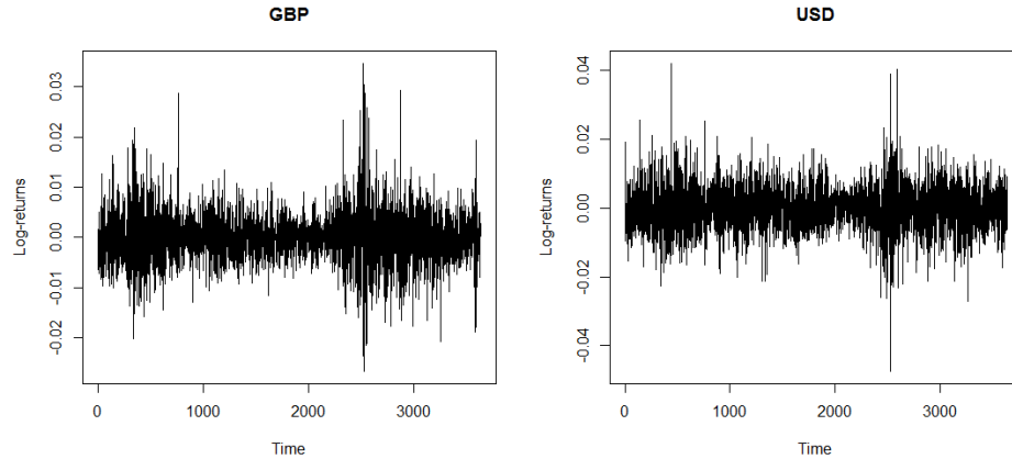
FIG. 5.1: The daily returns of the exchange rates of GBP and USD per one euro.
