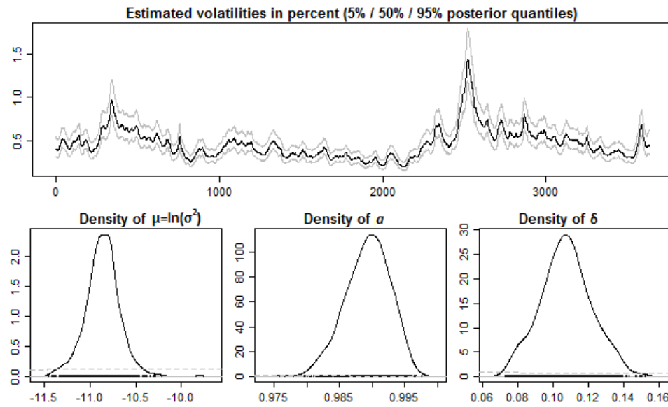
FIG. 5.2: Estimations of SV-parameters obtained by MCMC method (dataset is time series of daily returns of the exchange rates of GBP per one euro).
