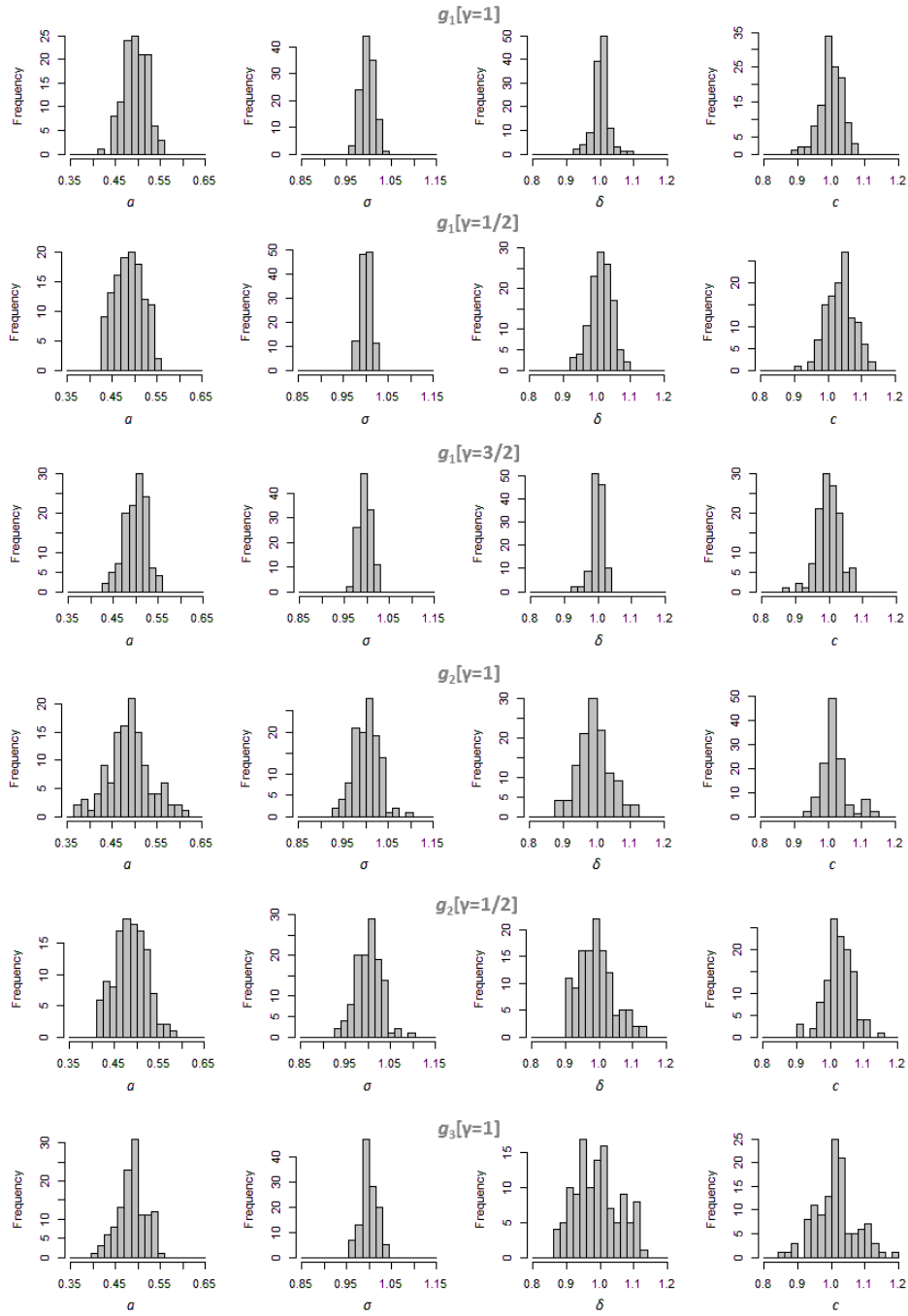
FIG. 4.2: Empirical distributions of estimated parameters, based on 120 MC simulations of Split-SV model
