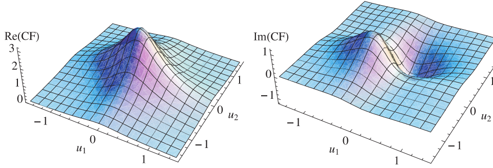
FIG. 3.1: Real and imaginary parts of two-dimensional CF of the sequence \mathbf{Y}_t^{(2)} = (Y_t, Y_{t+1}) .
