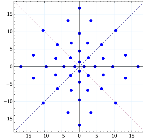
FIG. 4.1: Distribution of nodes in 44-point cubature formula of degree d = 15 for the weight function g_3 ( \gamma = 1 )
