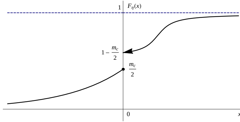
FIG. 1.1: The distribution function of CGD random variable.
