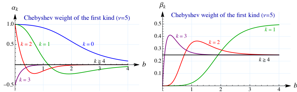
FIGURE 2. Three-term recurrence coefficients \alpha_k (left) and \beta_k (right) for \nu = 5
